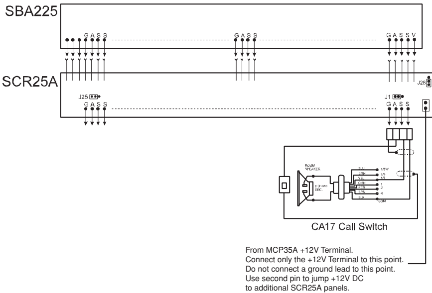
Model CA17 Connecting Diagram
